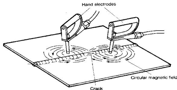
Magnetization using hand held electrodes.
