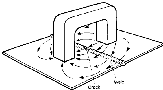
Magnetization using a permanent magnet.
